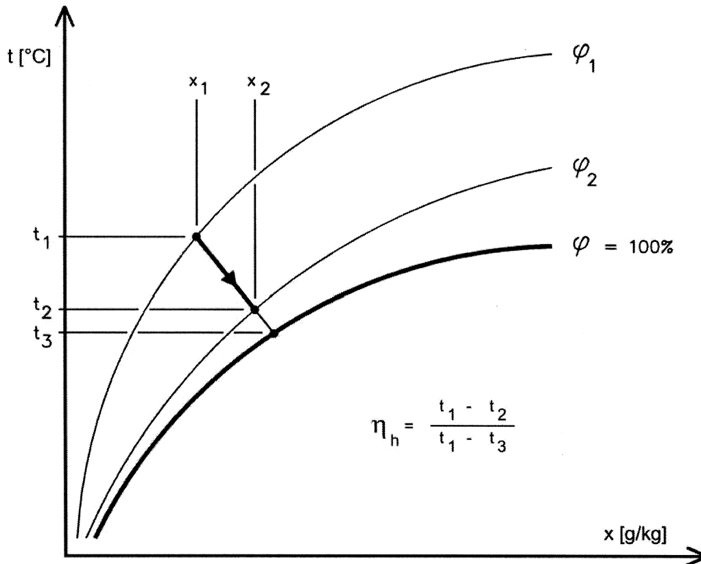
Figure 9 — Humidifier efficiency
